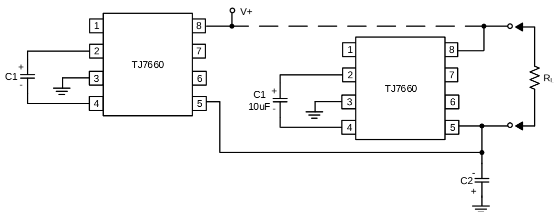
Figure 15. Paralleling Devices
